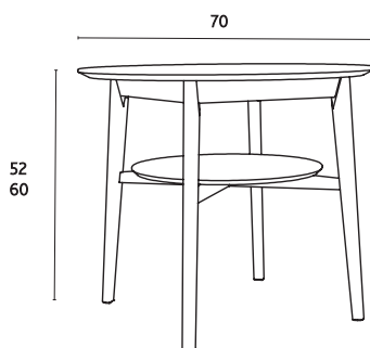
6120/6220 EMMA 6120U/6220U EMMA (Utan hylla/Without shelf)
