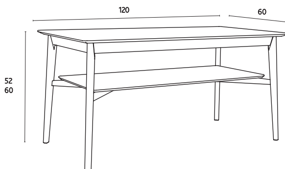
6131/6231 EMMA 6131U/6231U EMMA (Utan hylla/Without shelf)
