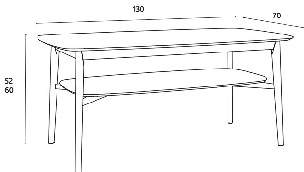
6130/6230 EMMA 6130U/6230U EMMA (Utan hylla/Without shelf)
