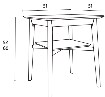
6130/6230 EMMA 6130U/6230U EMMA (Utan hylla/Without shelf)
